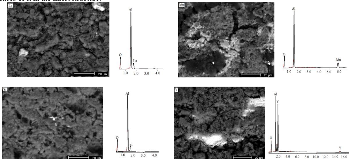
Figure 4. SEM microstructure of different manufactured composite.
